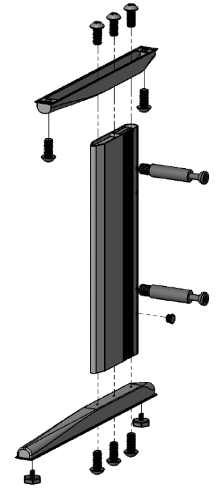
LEG ASSEMBLY
